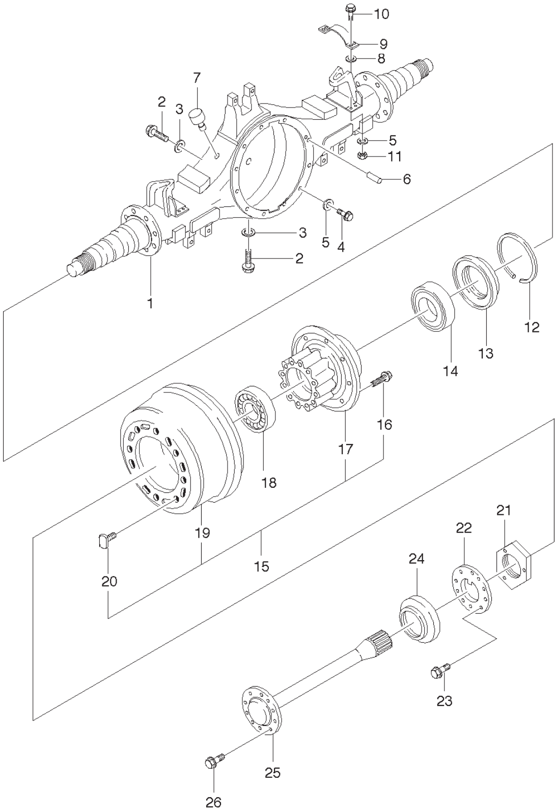
REAR AXLE CASE FORWARD
