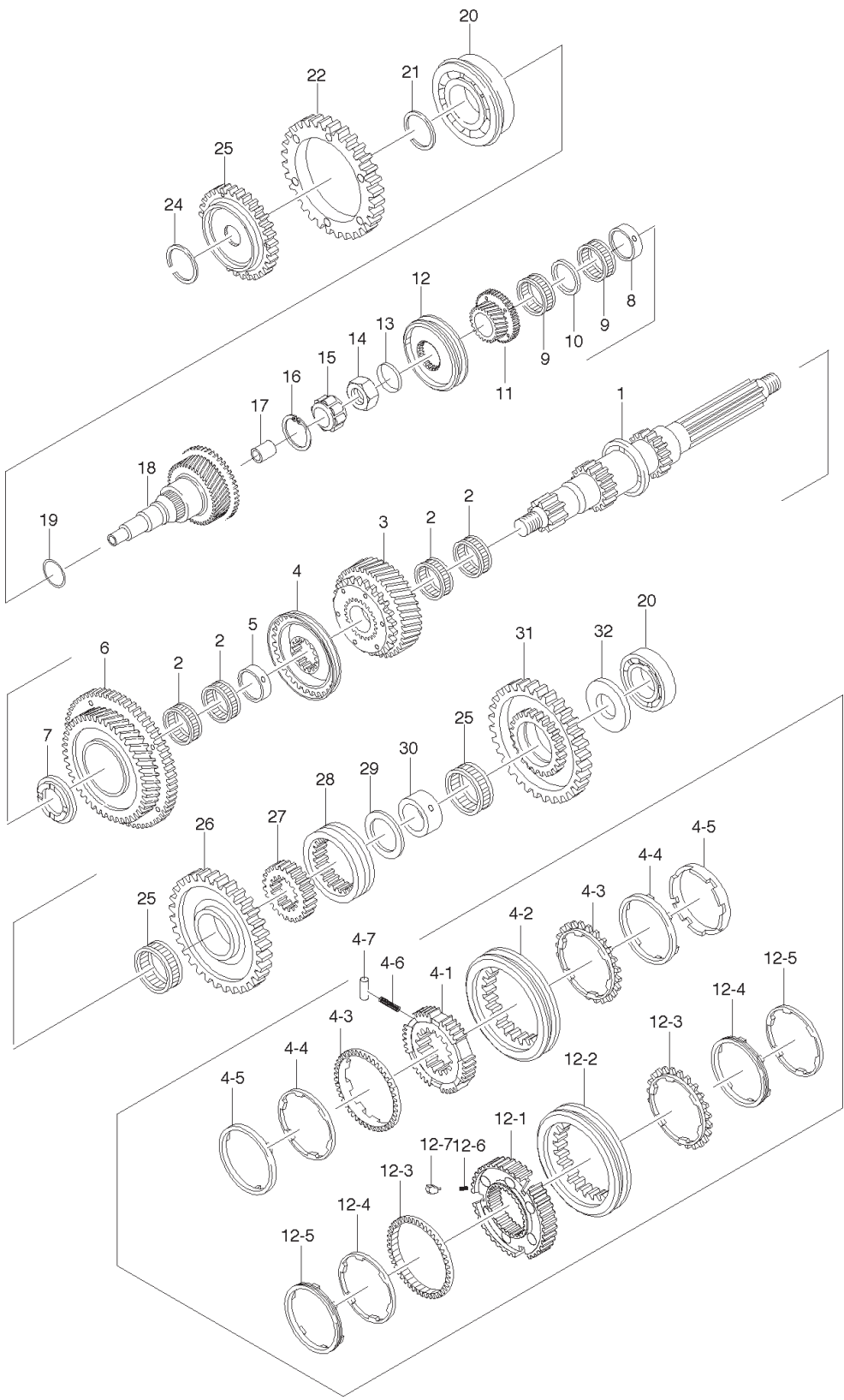
TRANSMISSION GEAR
